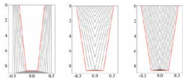
FIG. 8. Schematic filling of a trench starting with superconformal growth, SC = 2 (left), followed by continued superconformal growth (center) or by conformal growth, SC = 1 (right). Reprinted with permission from Wang and Abelson, J. Appl. Phys. 116 , 194302 (2014). Copyright 2014, AIP Publishing LLC.
